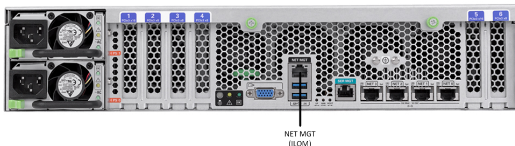
Figure 2-5 Connecting to ILOM Port
