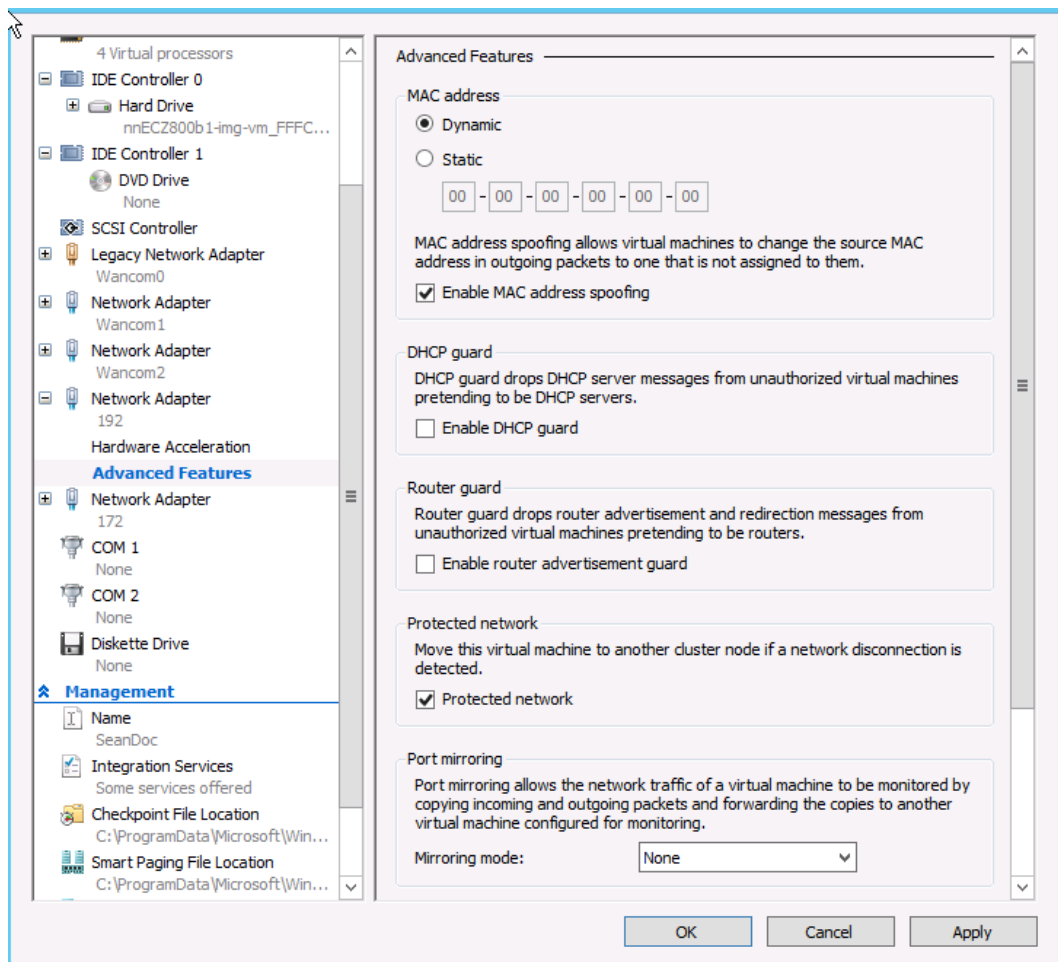
Figure 6-1 VM Settings on Hyper-V
