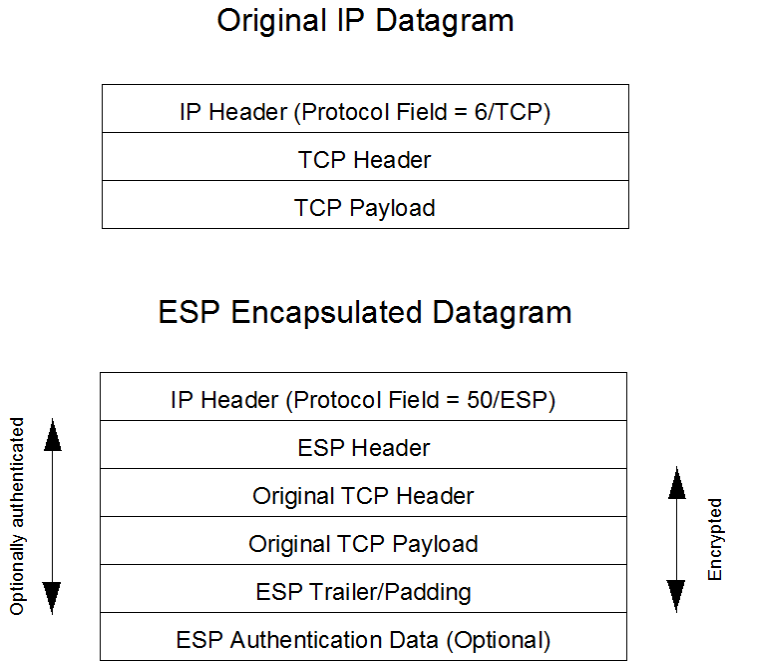
Figure 14-3 ESP Transport Mode
