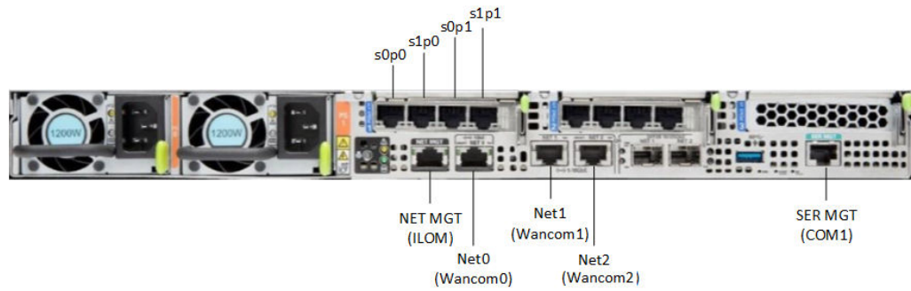
Figure 4-11 Oracle X8-2 Configuration A (4x10 GigE NIC)
