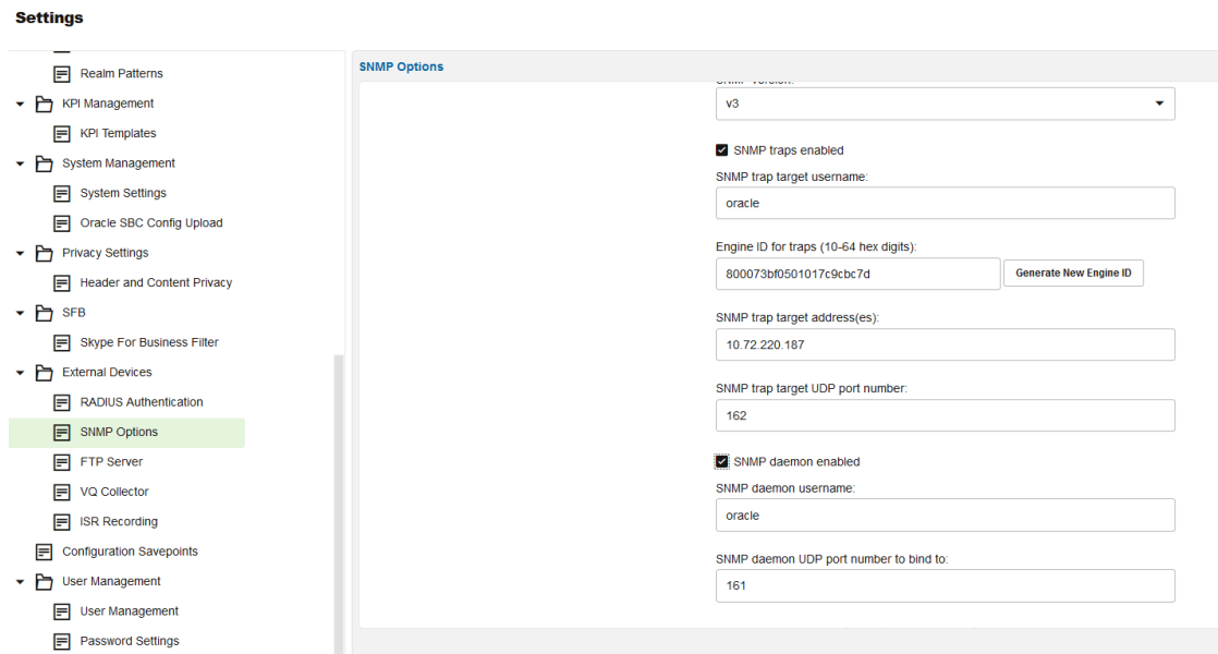
Figure 7-34 SNMP Options
