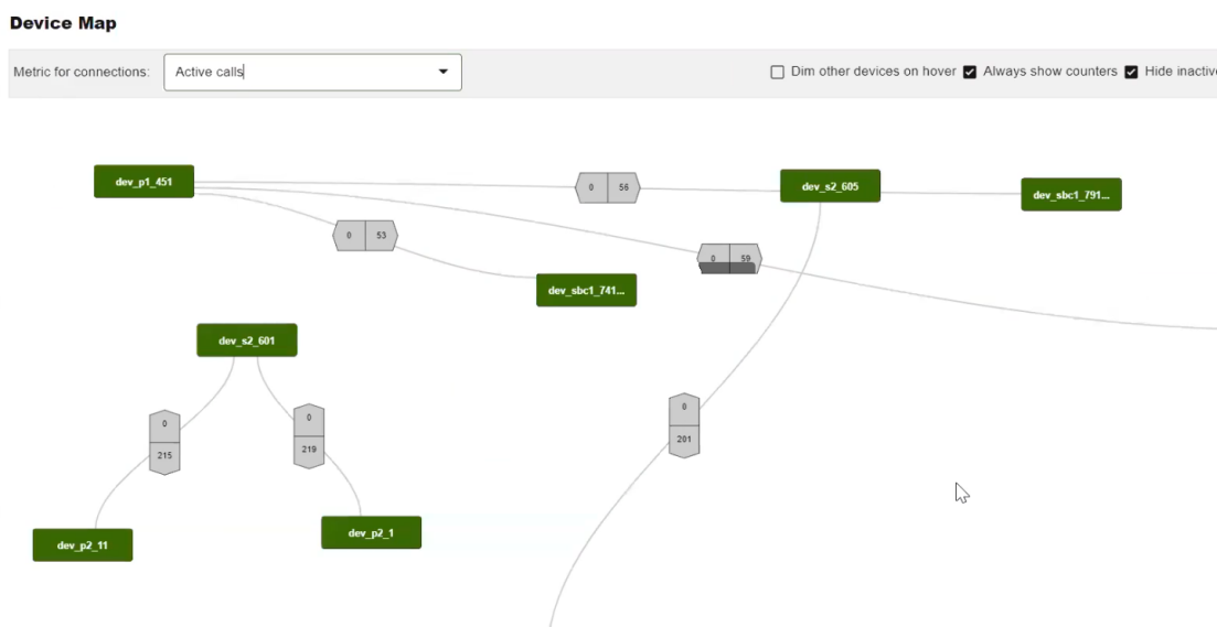
Figure 4-77 Device Map
