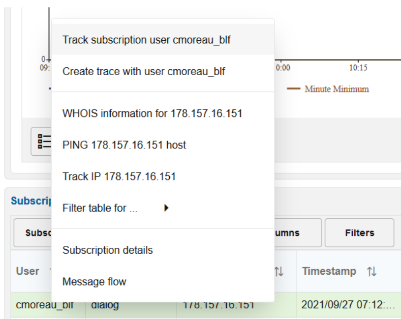
Figure 4-63 Subscriptions Table
