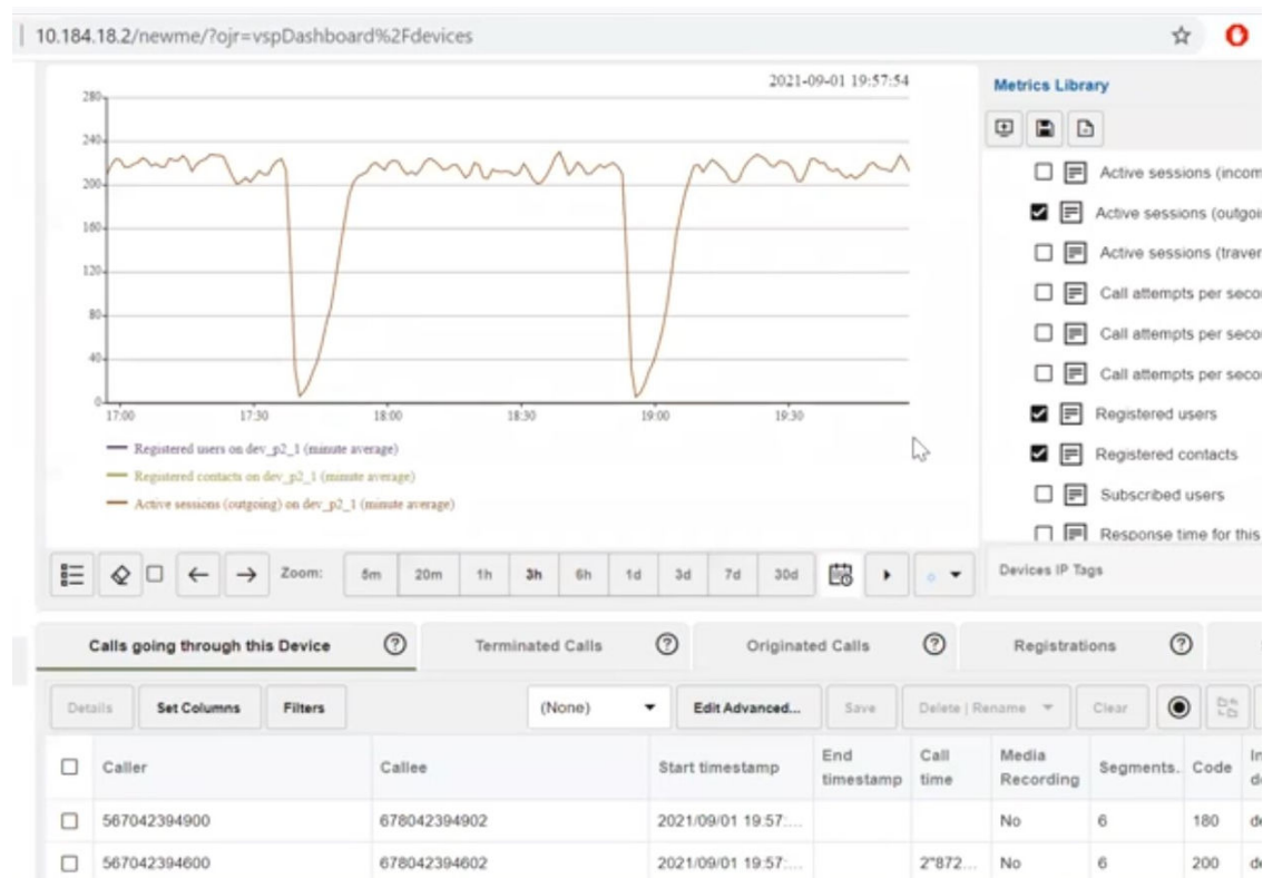
Figure 4-76 Devices Page
