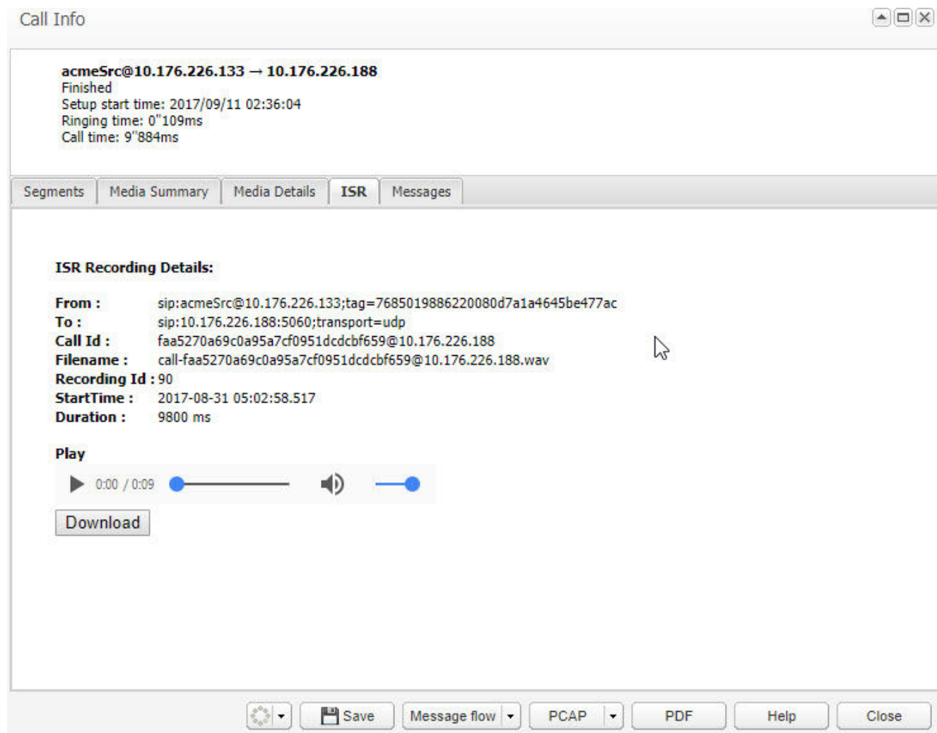
Figure 4-35 ISR Tab
