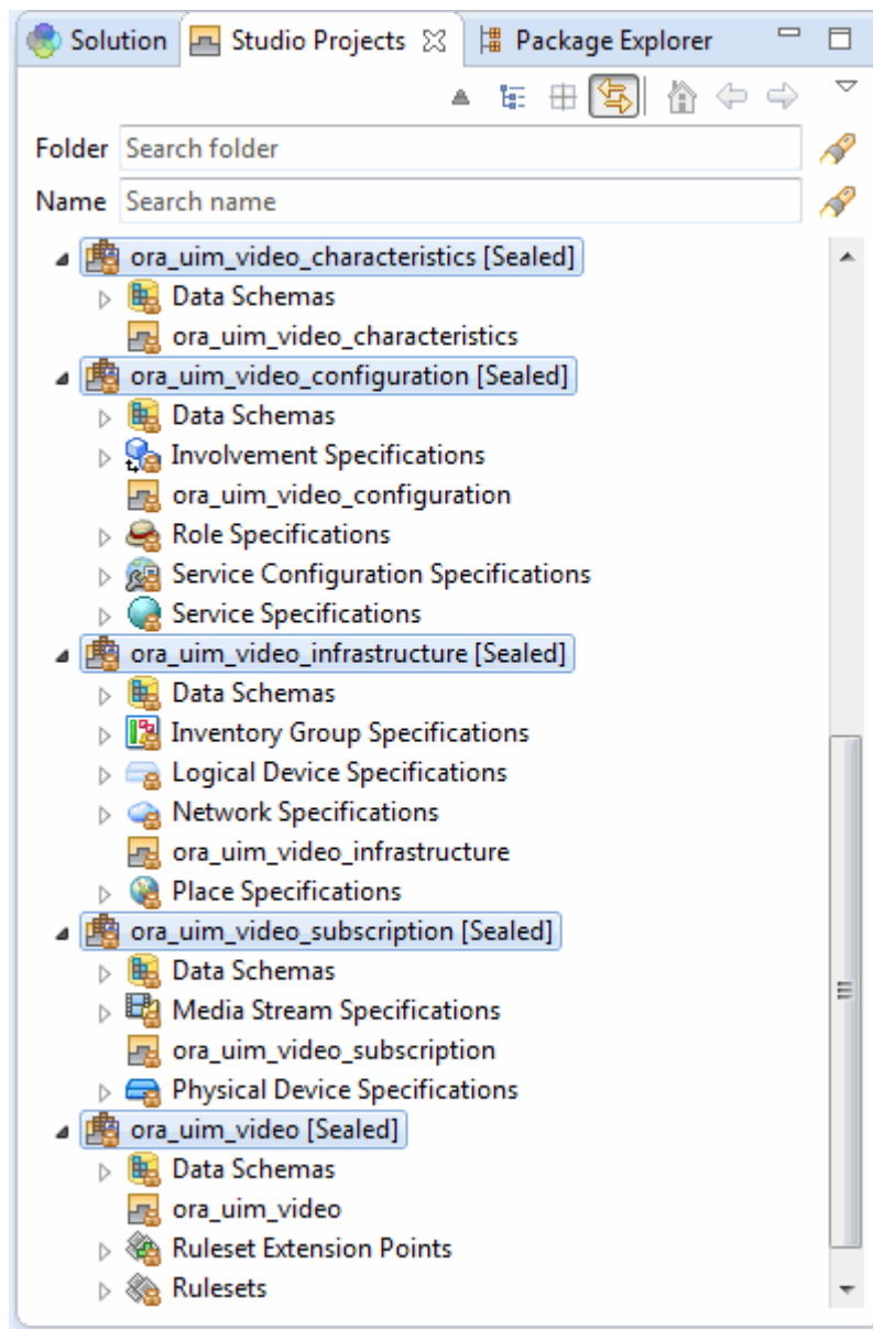
Figure 2-1 Imported Cartridge Packs
