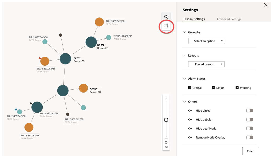
Figure 5-1 Display Settings panel in UTIA
