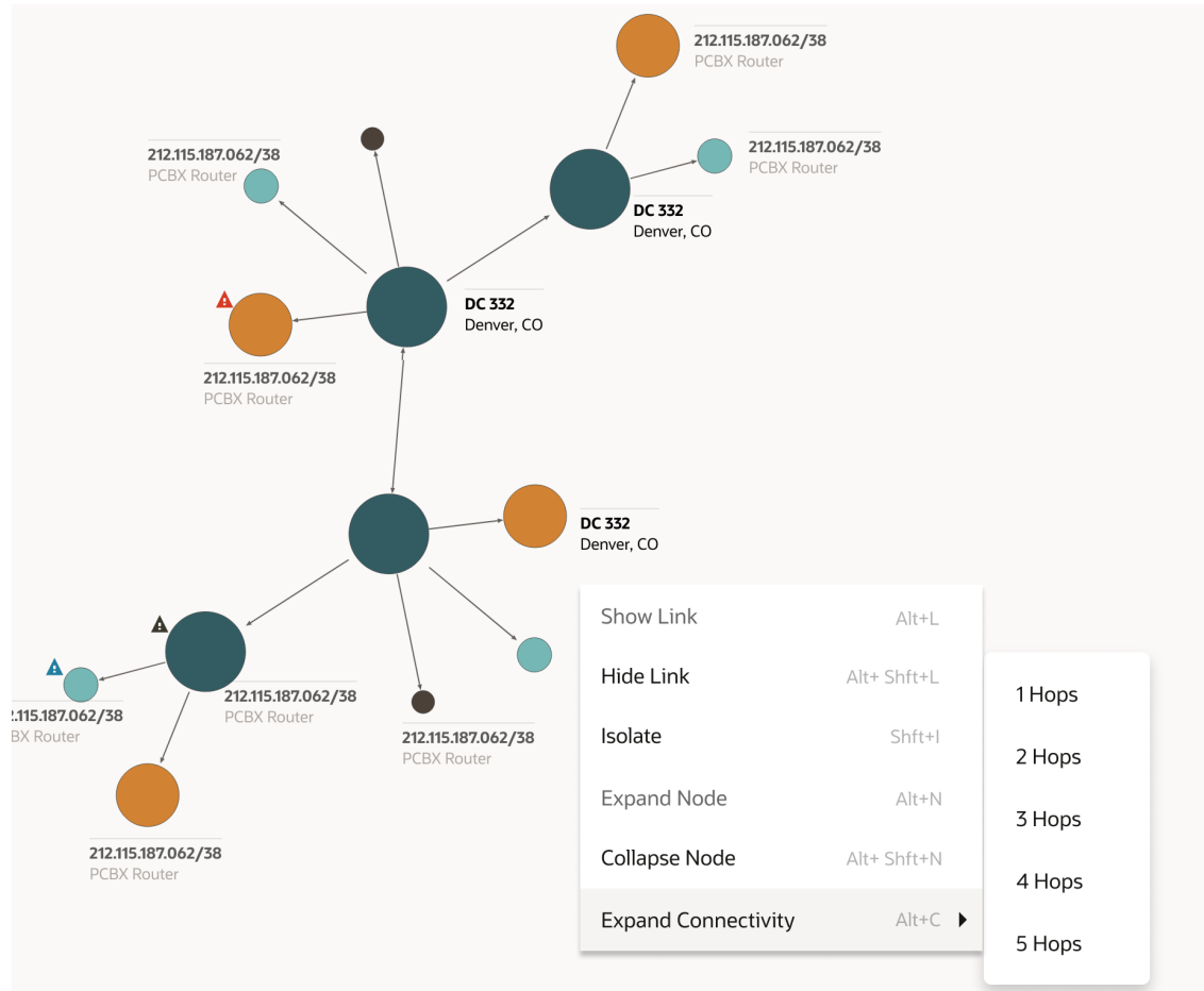
Figure 6-1 Context menu options in UTIA
