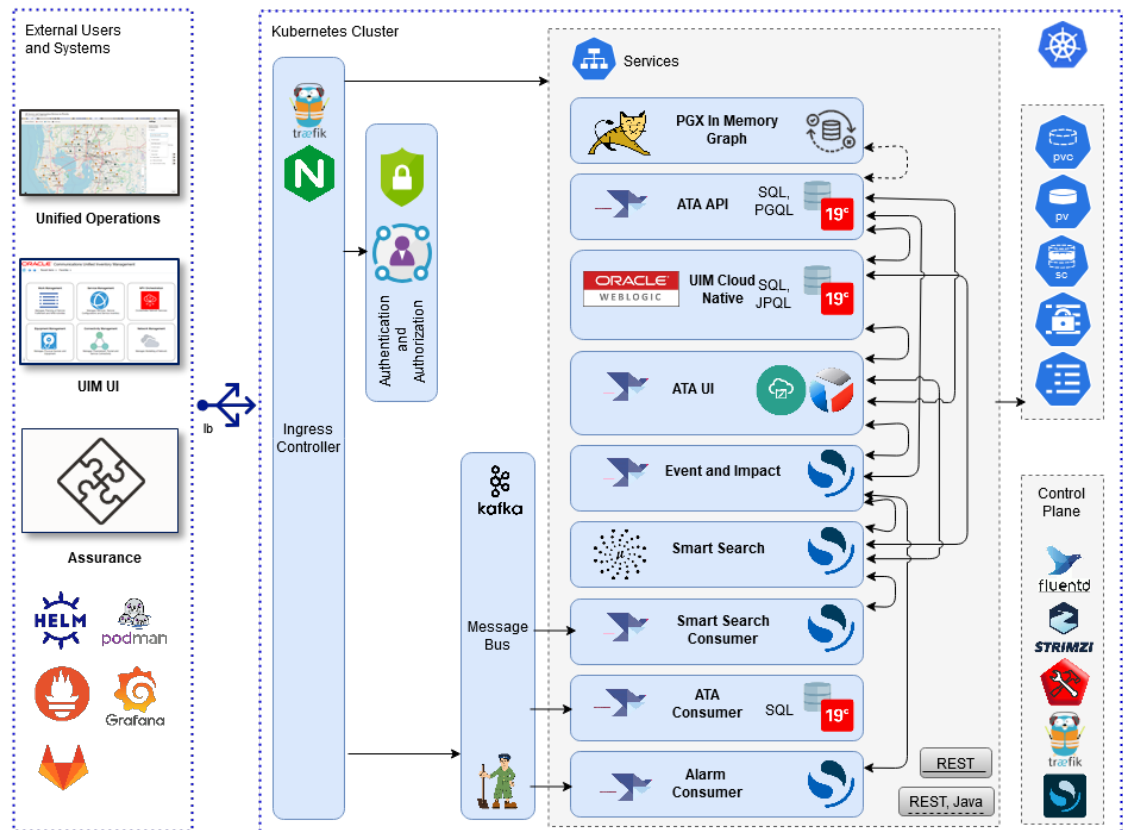
Figure 8-1 ATA Architecture
