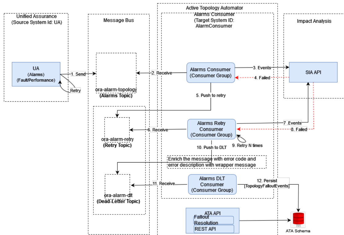
Figure 8-3 Fallout Events Resolution for Alarm Consumer
