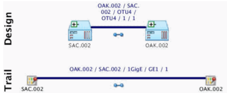
Figure 14-14 Schematic View of 1GigE Connectivity Enabled by OTN Connectivity
