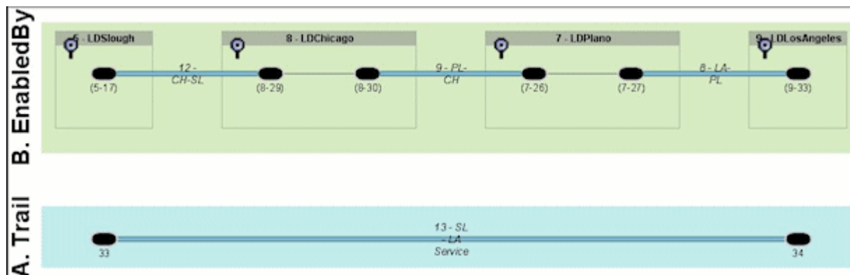
Figure 17-21 Pipe Enablement
