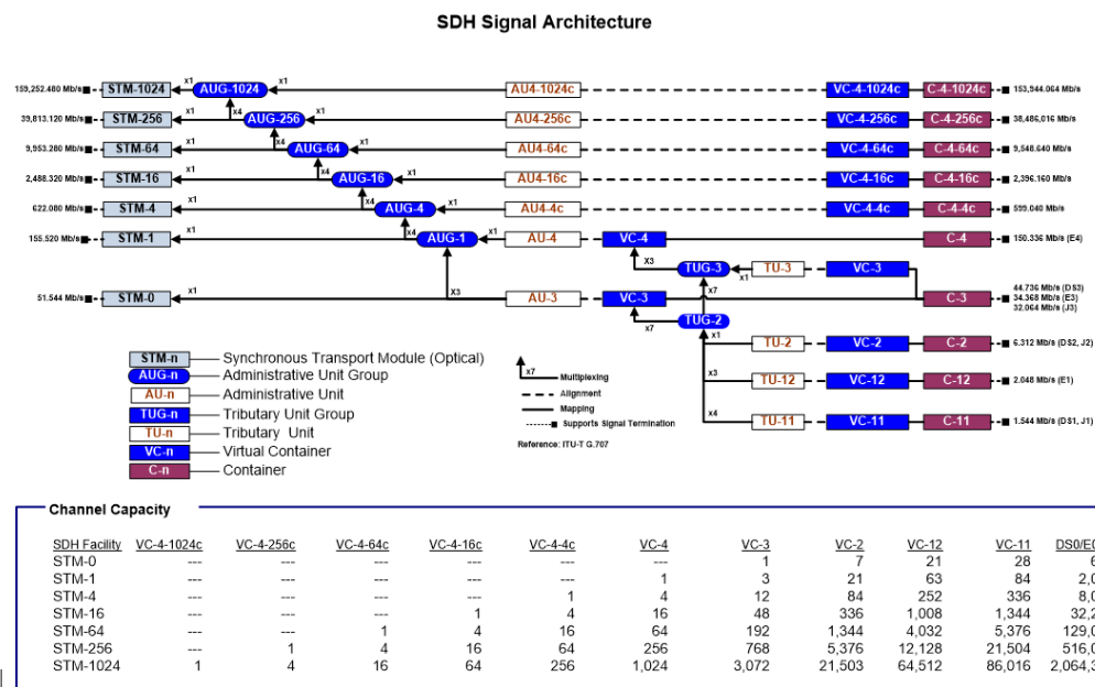
Figure 14-6 SDH Signal Hierarchy
