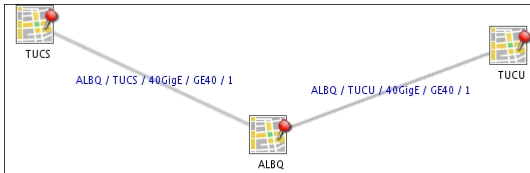
Figure 15-2 Transport Network
