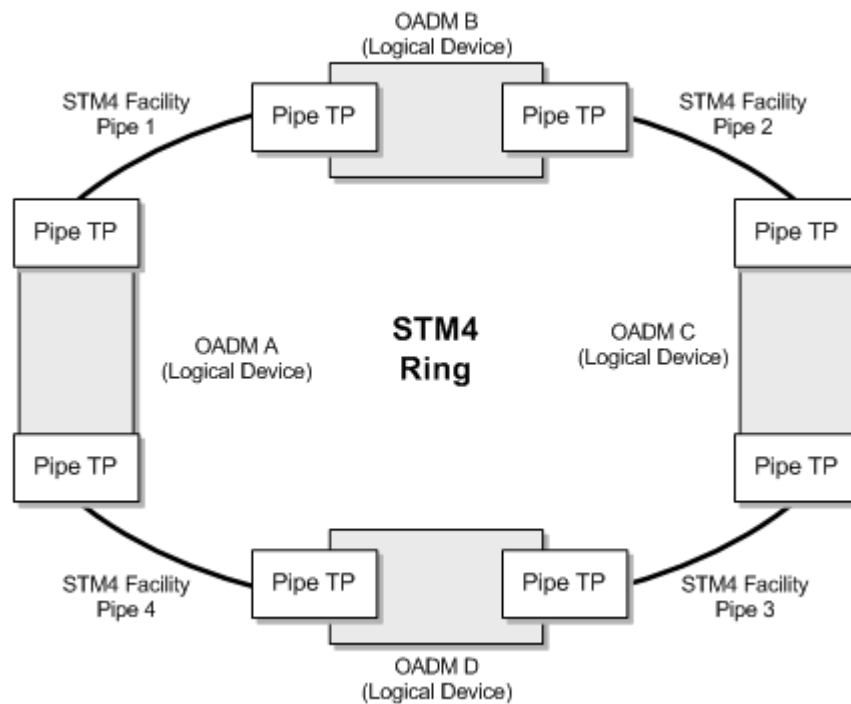
Figure 17-4 STM4 Ring
