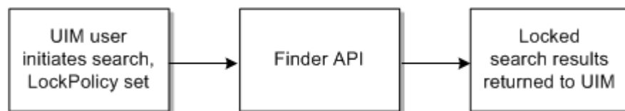
Figure 13-2 Flow of Entity Finder API with Row Locking
