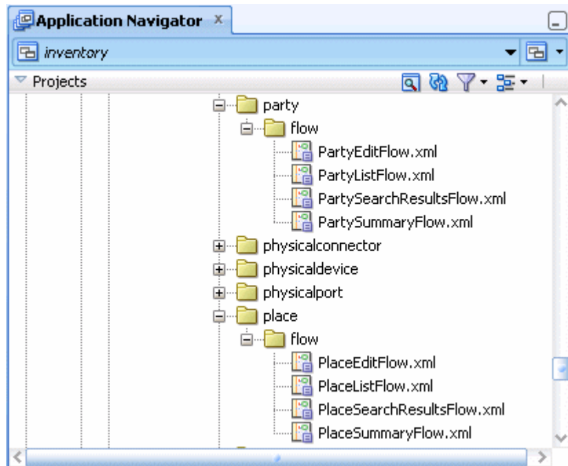
Figure 11-3 Task Flow File Naming Conventions
