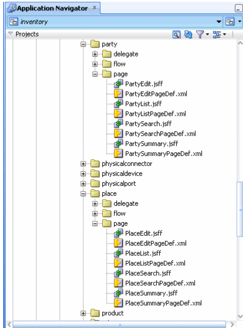
Figure 11-2 Page File Naming Conventions
