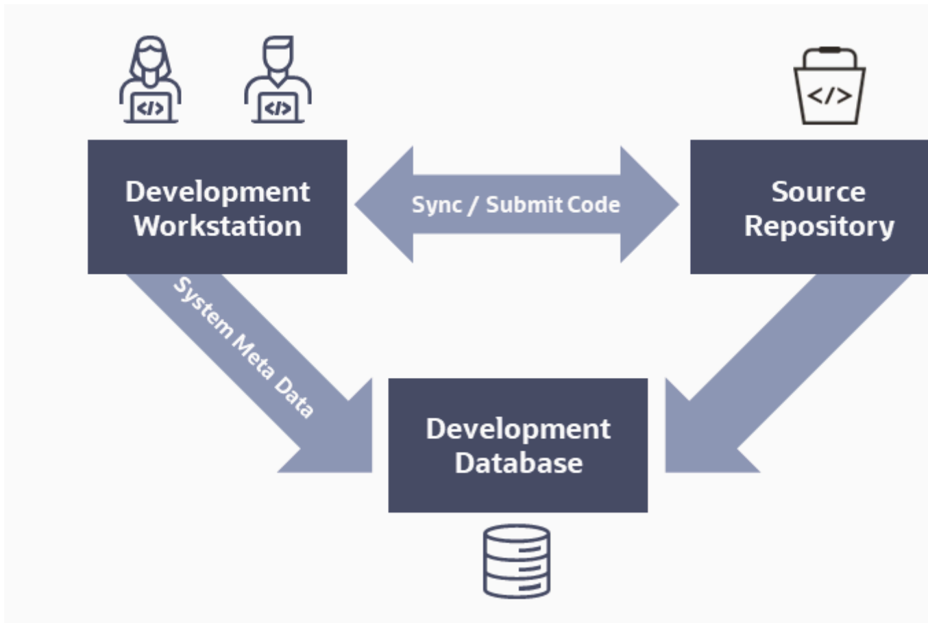
Development Environment
