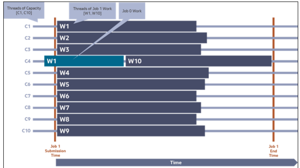
Figure 3-2: Coarse-Grained Submission - Delayed Job Completion
