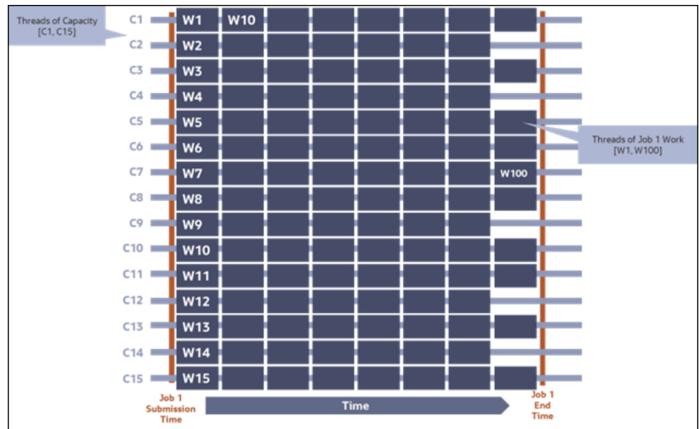
Figure 3-6: Fine-Grained Submission - Excess Capacity Shortens Completion Times
