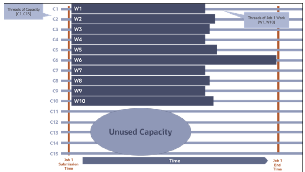
Figure 3-3: Coarse-Grained Submission - Unused Capacity
