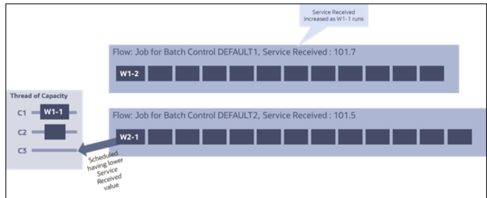
Figure 3-8: Two Flows - More Thread Capacity
