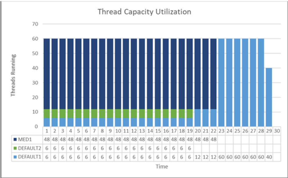
Figure 3-10: Thread Capacity Utilization
