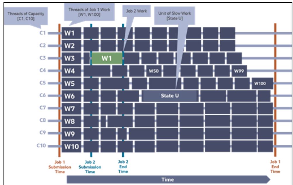
Figure 3-4: Fine-Grained Submission
