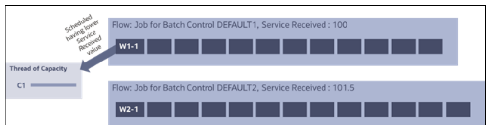
Figure 3-7: Two Flows
