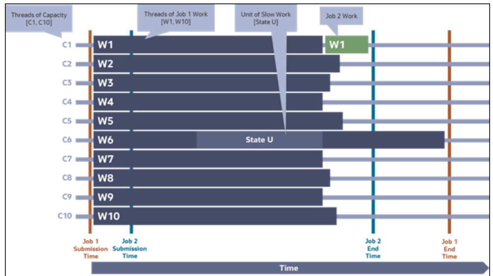
Figure 3-1: Coarse-Grained Submission - Two Jobs
