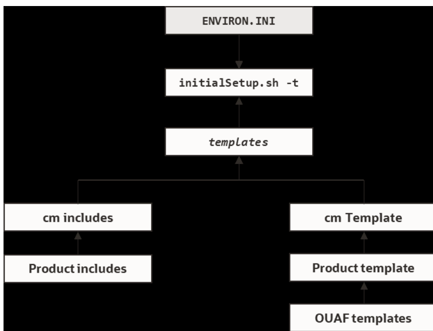
Figure 35 – Template Hierarchy
