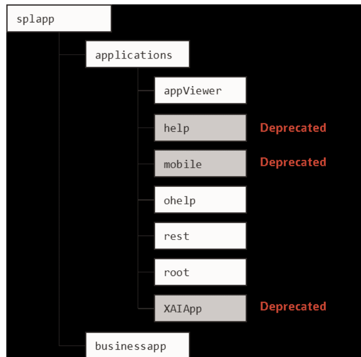
Figure 33 – Expanded Format
