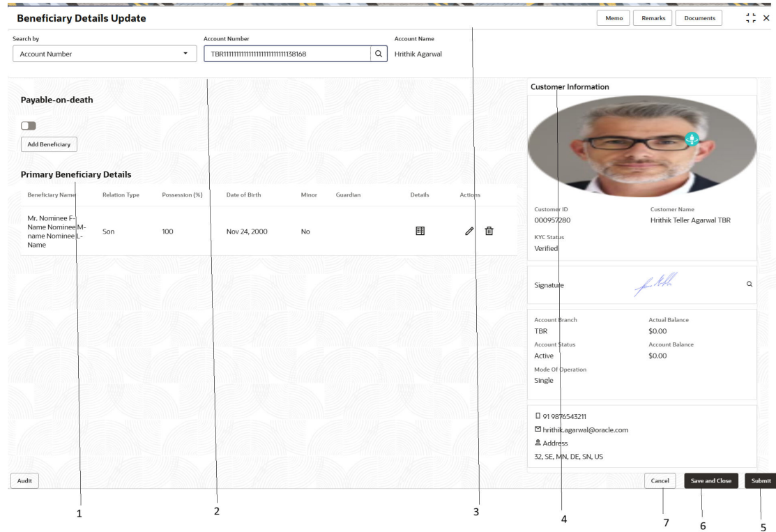
Figure 3-3 Beneficiary Details Update
