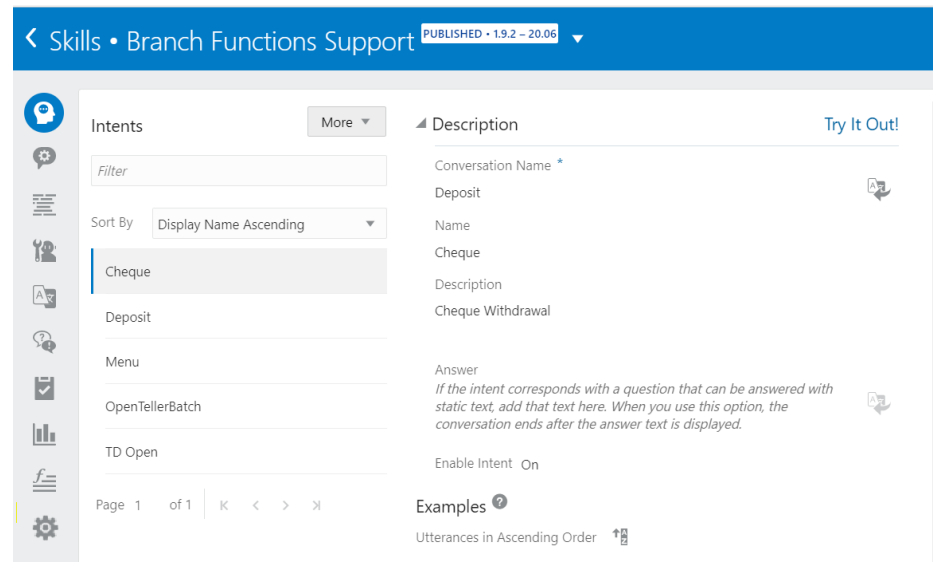
Figure 16-4 Select Skill
