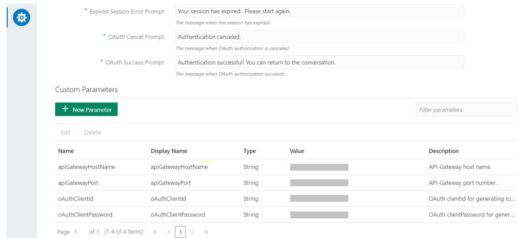
Figure 16-6 Custom Parameters
