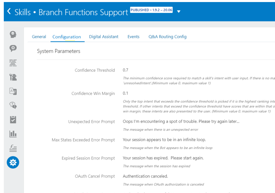
Figure 16-5 Skills - Configuration
