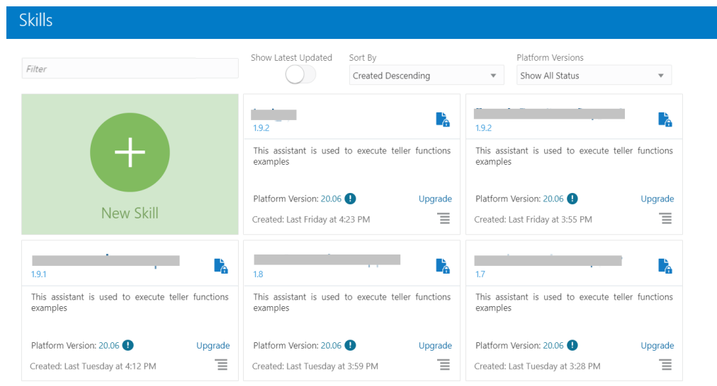
Figure 16-3 Skills
