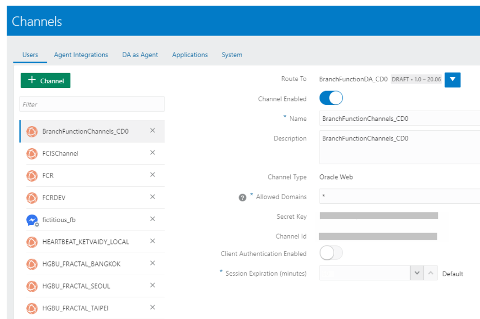
Figure 16-9 Channels
