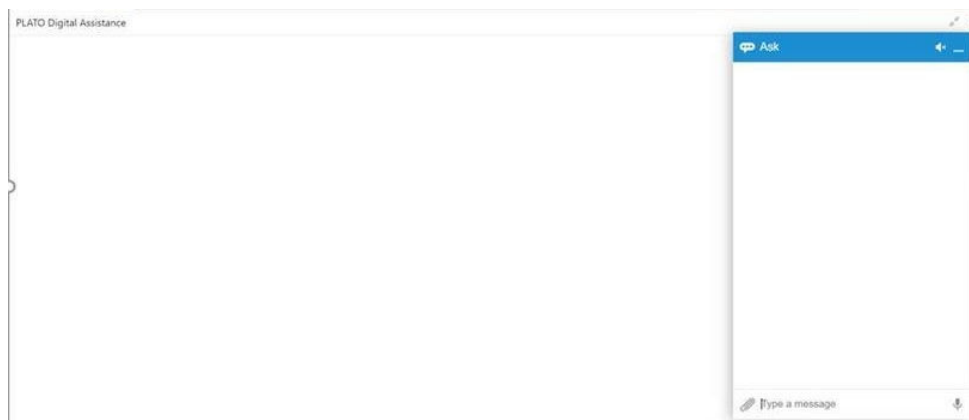
Figure 16-2 Chatbot
