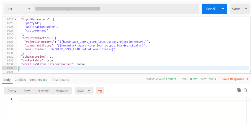
Figure 14-3 Response Status
