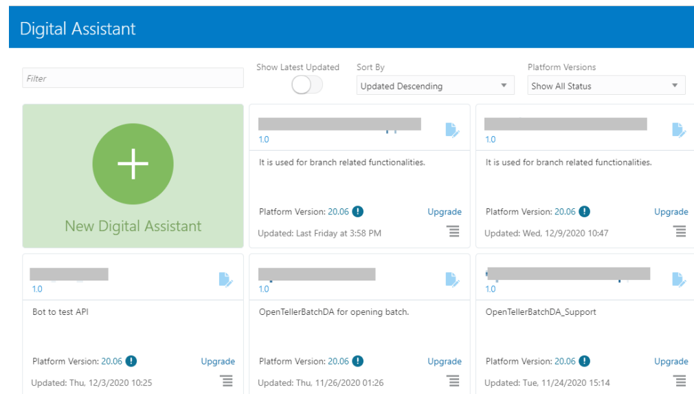
Figure 16-7 Digital Assistants
