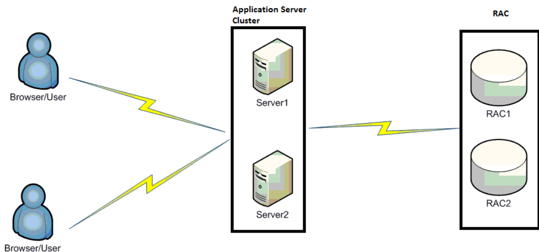
Figure 1-1 Centralized
