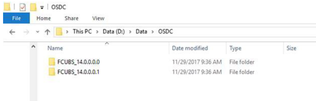
Figure 1-2 Folder Structure
