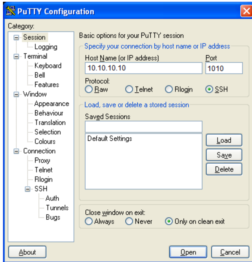
Figure 1-6 PuTTY Configuration
