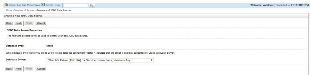
Figure 7-6 JDBC Data Source Properties
