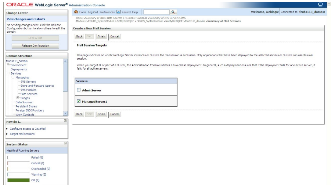
Figure 7-81 Create a New Mail Session - Targets
