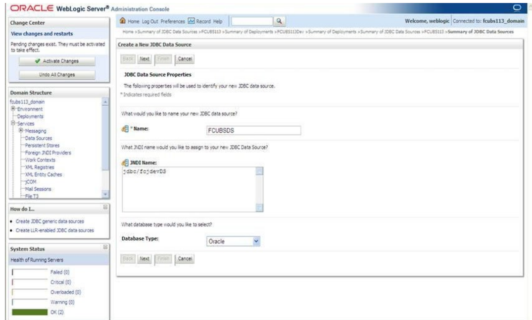
Figure 7-18 Create a New JDBC Data Source
