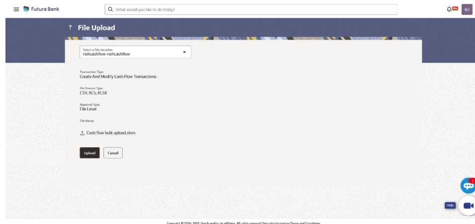
Figure 4-13 File Upload - Post Uploading File
