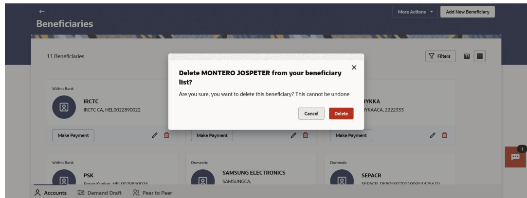
Figure 2-21 Delete Payee
