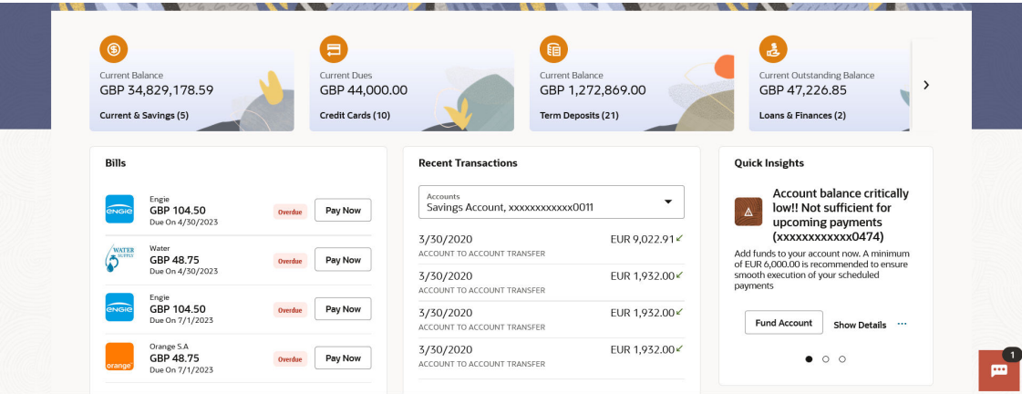
Figure 1-1 Overview widget
