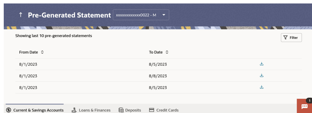
Figure 16-4 Pre-generated Statements
