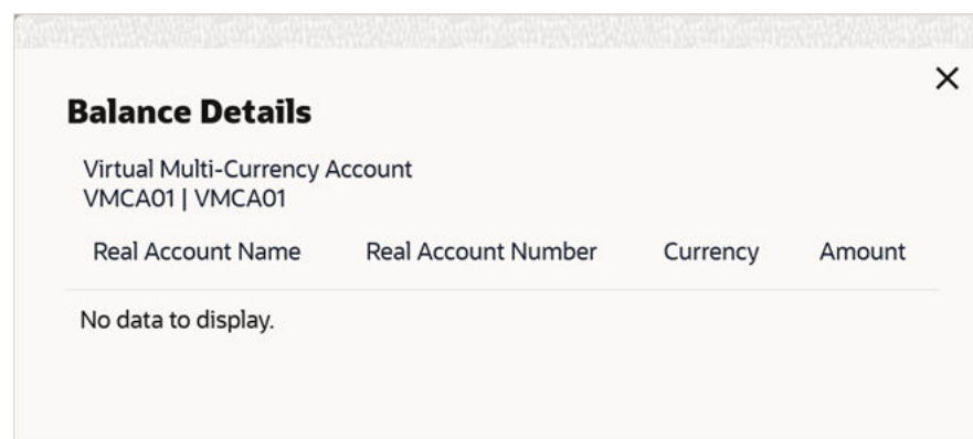
Figure 6-6 Balance Details
