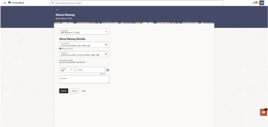
Figure 12-1 Move Money
