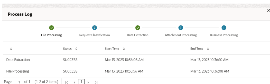
Figure 4-23 Process Log
