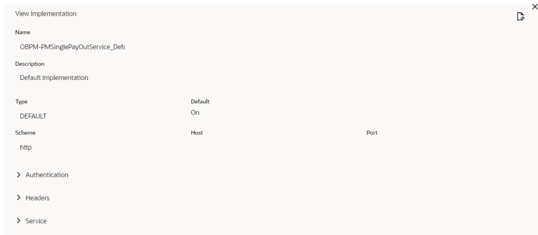
Figure 2-57 Equifax Sandbox
