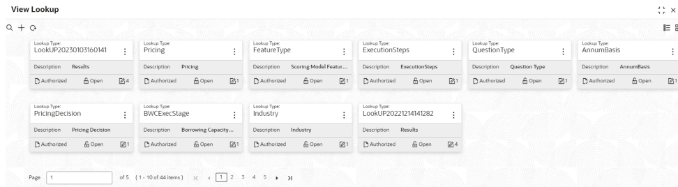
Figure 3-9 View Lookup
