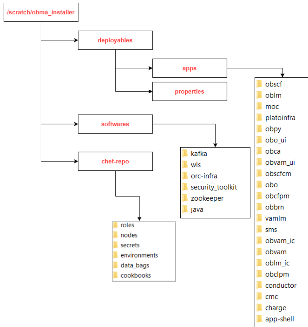
Figure 3-1 Installer Folder Structure
