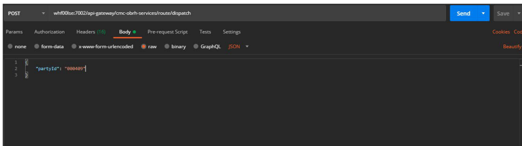
Figure 17-5 Request Payload
