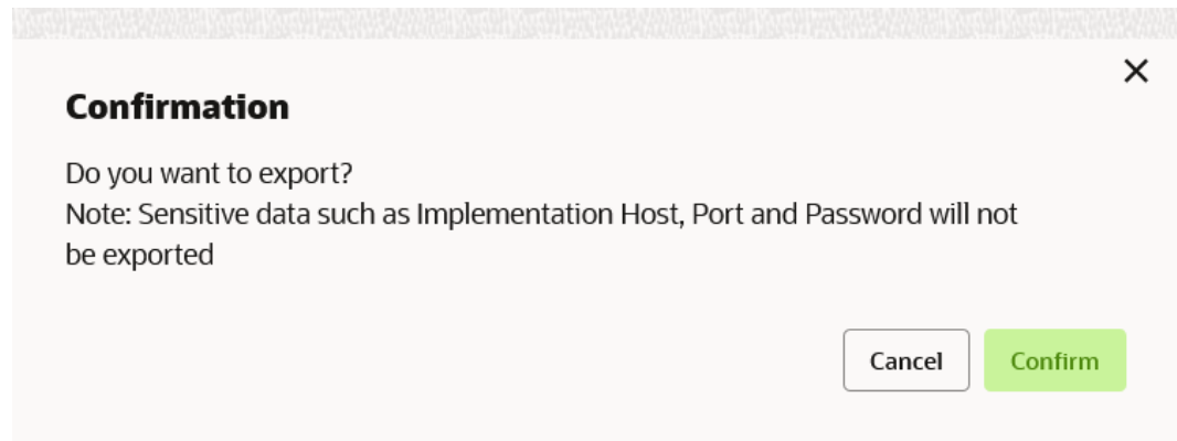
Figure 2-14 Confirmation
