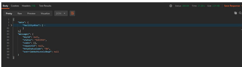
Figure 17-6 Response Payload on Successful Dispatch
