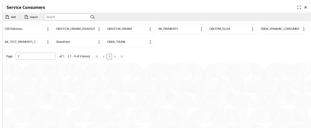
Figure 2-1 Service Consumers
