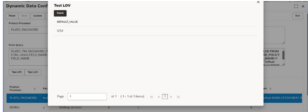
Figure 9-43 Test LOV
