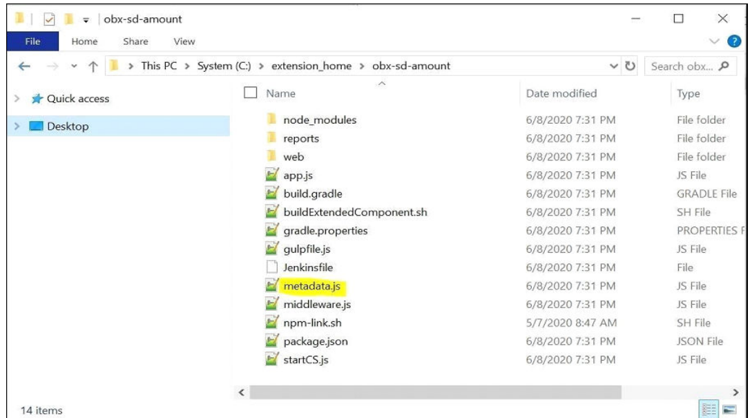
Figure 4-8 obx-sd-amount
