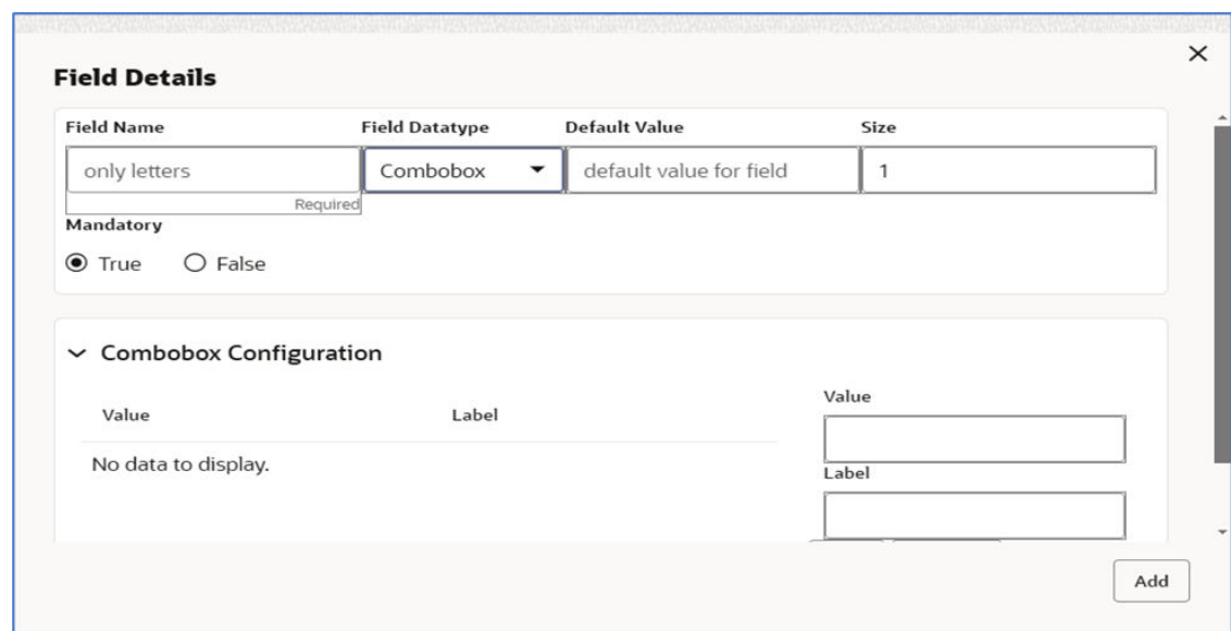
Figure 2-9 Combobox Configuration
