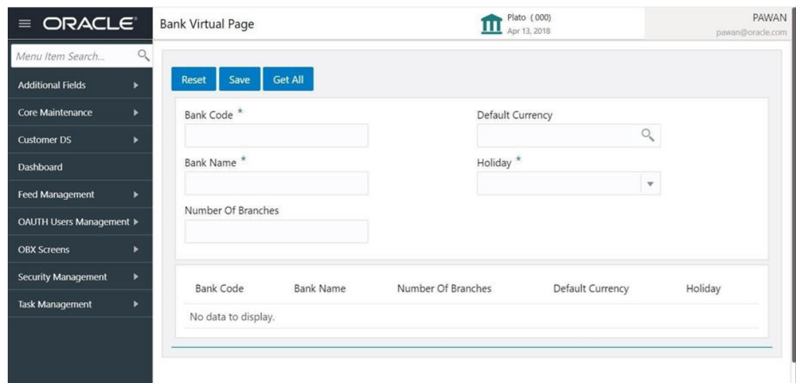
Figure 4-1 Virtual Page
