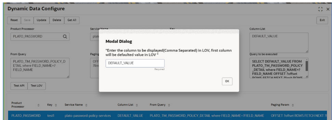
Figure 9-42 Modal Dialog
