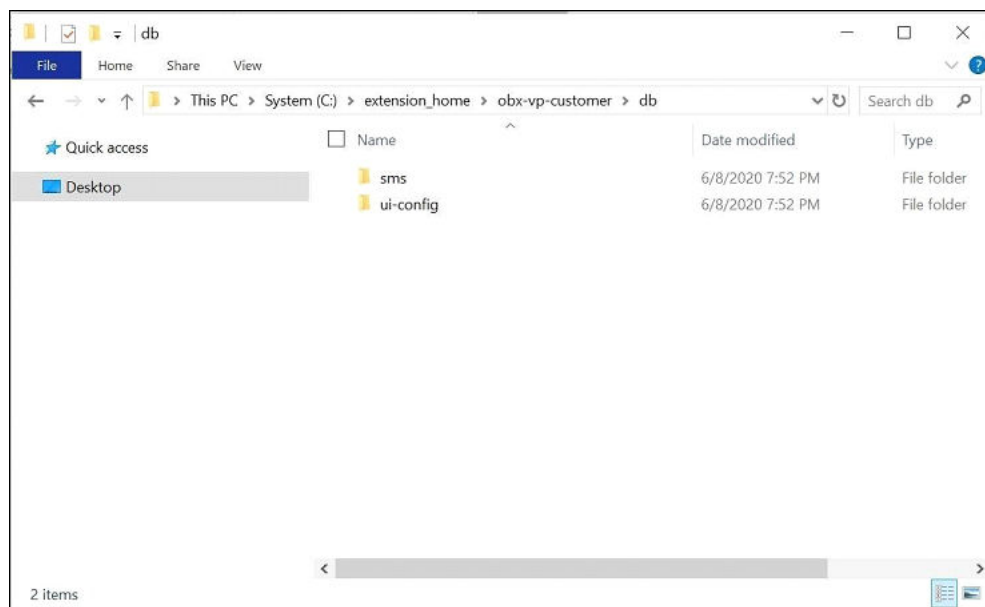
Figure 4-29 DB Folder
