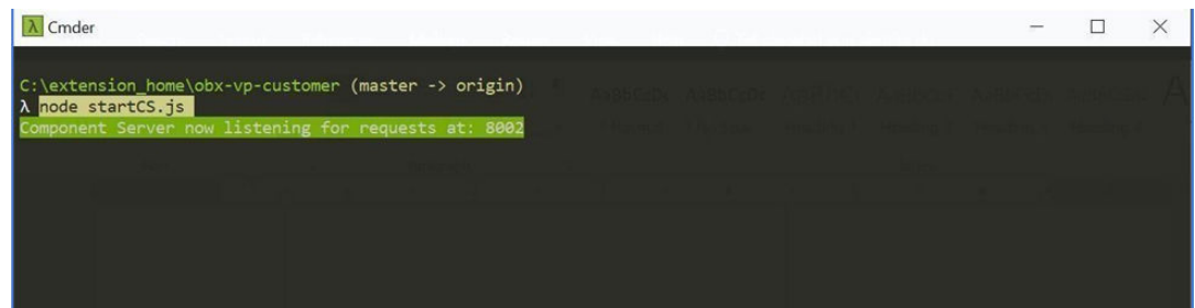
Figure 4-25 Node startCS.js
