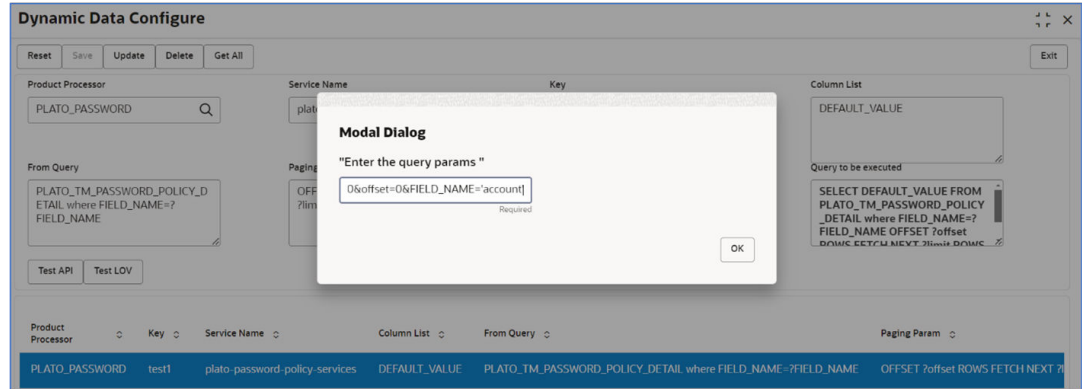
Figure 9-40 Modal Dialog
