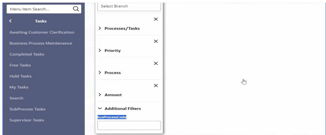
Figure 9-45 Screen UI
