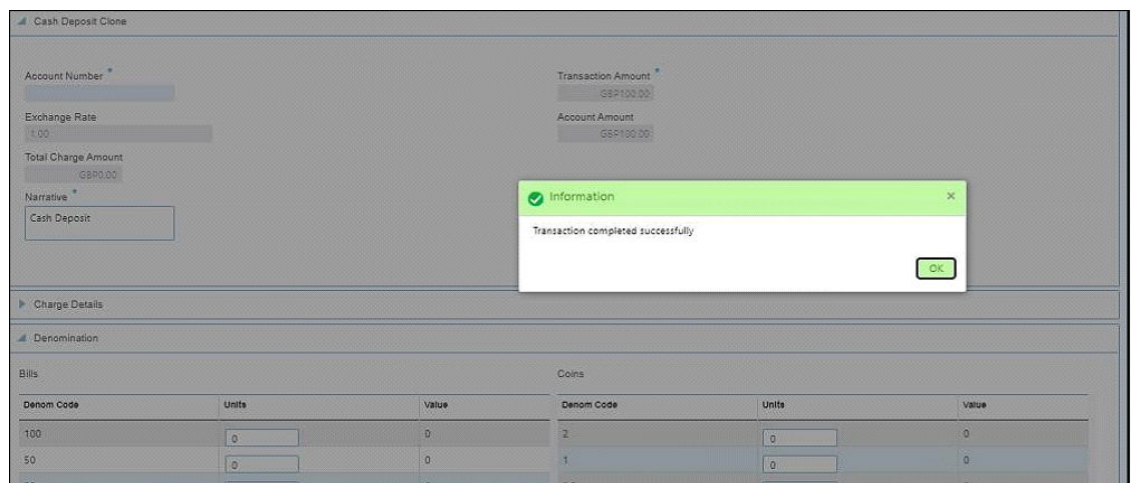
Figure 9-2 Information Message
