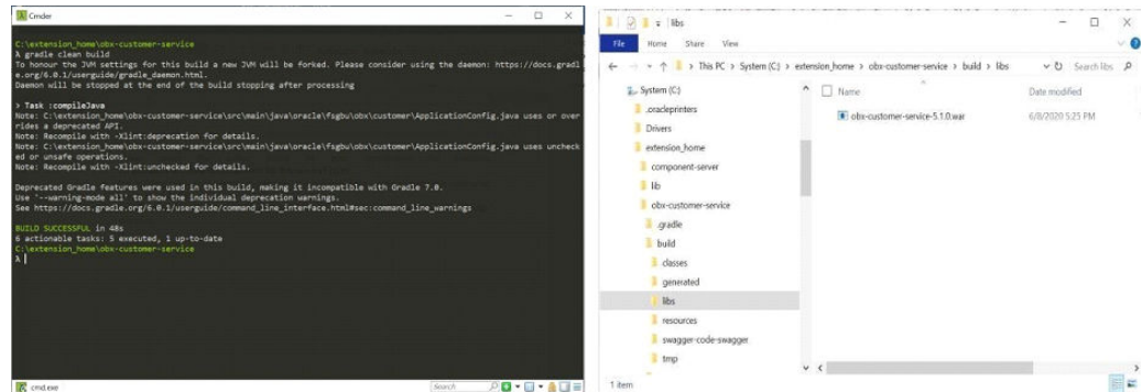
Figure 3-19 Lib's Directory
