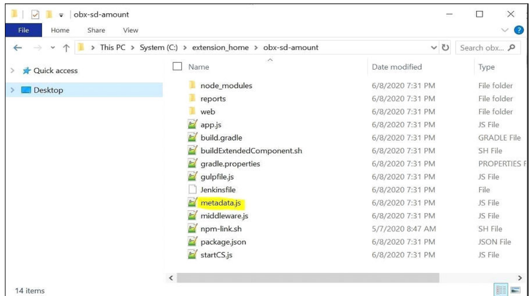
Figure 4-8 obx-sd-amount
