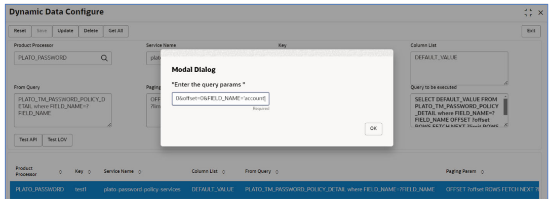
Figure 9-41 Modal Dialog
