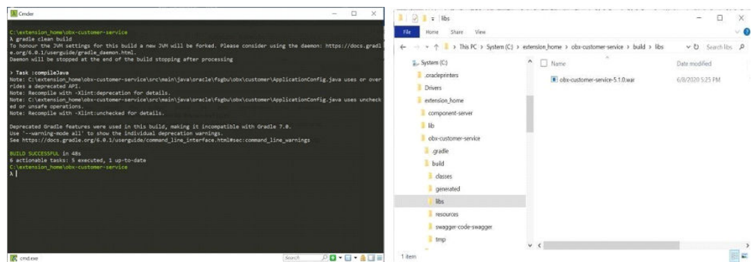
Figure 3-6 Lib's Directory
