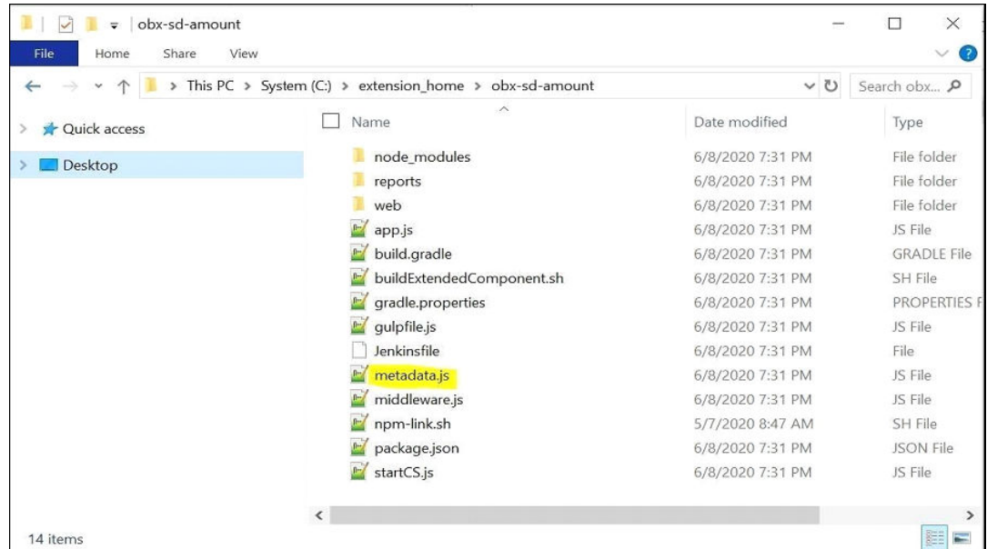
Figure 4-13 obx-sd-amount
