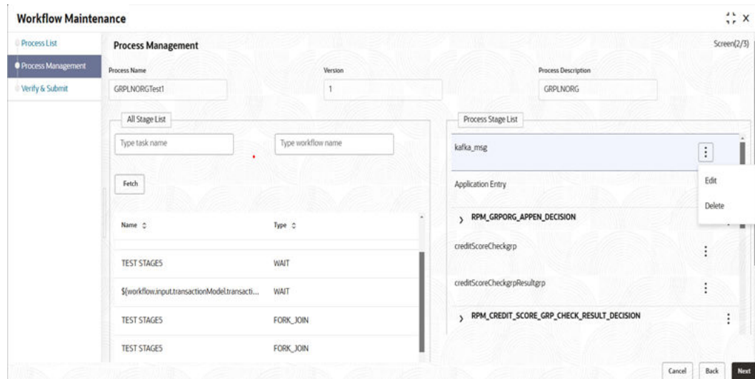
Figure 5-6 Process management
