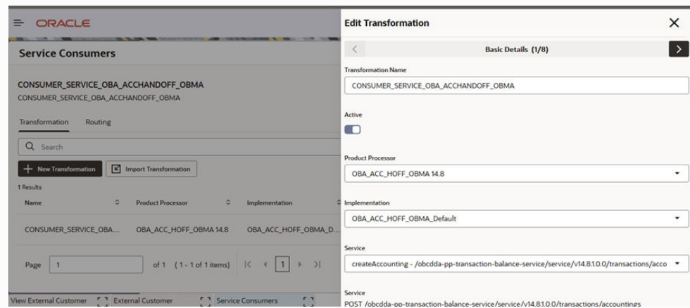
Figure 6-6 Service Consumer
