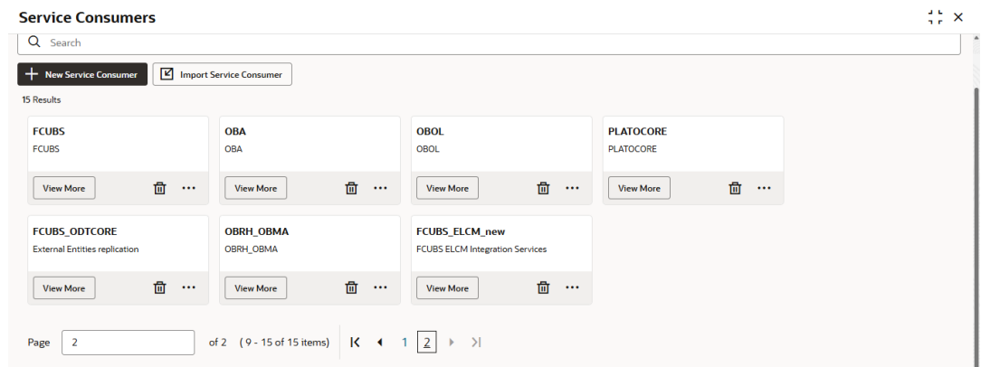
Figure 6-7 Service Consumer
