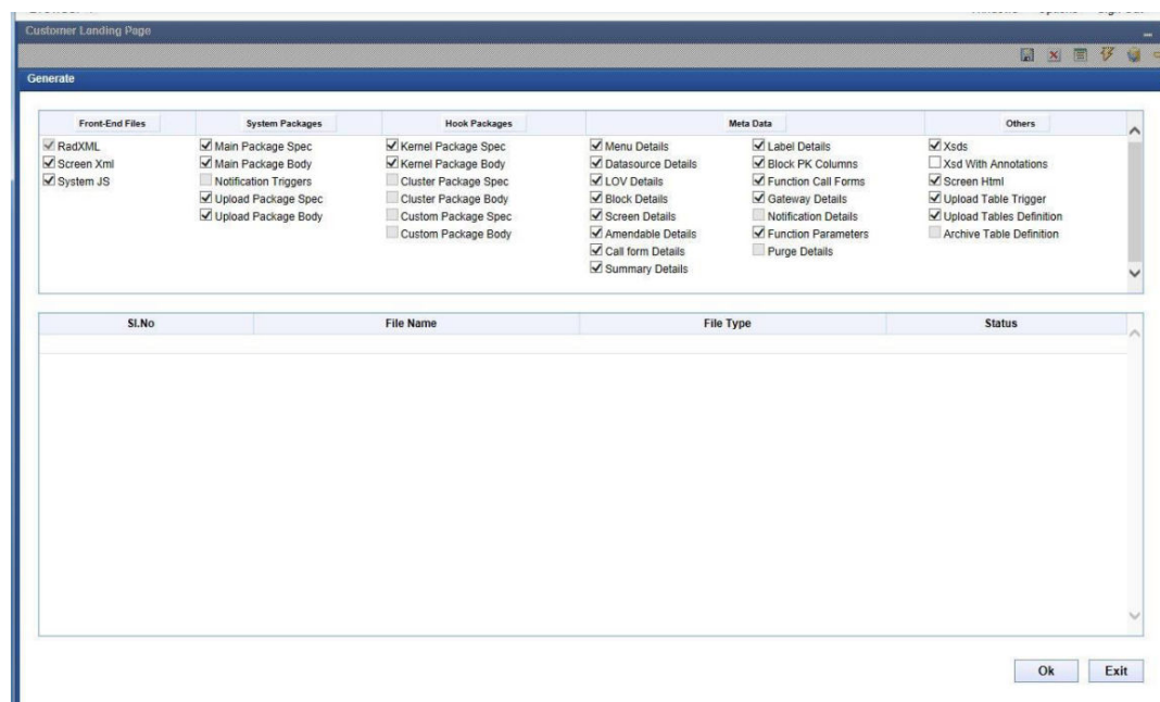
Figure 3-8 Generate
