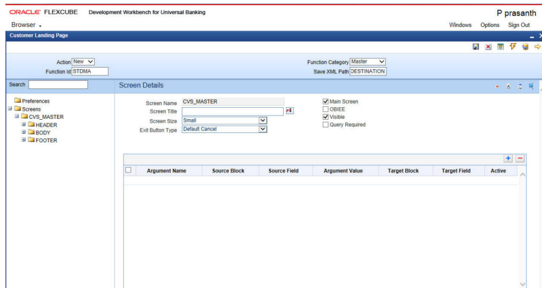
Figure 3-4 Screen Details
