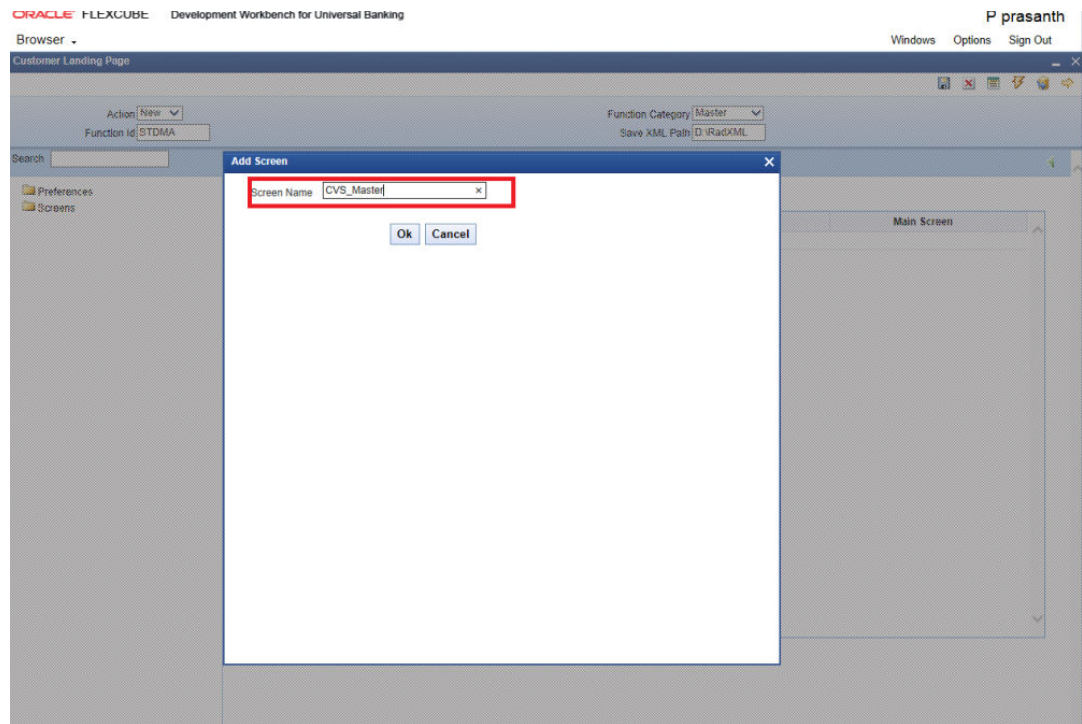
Figure 3-3 Add Screen
