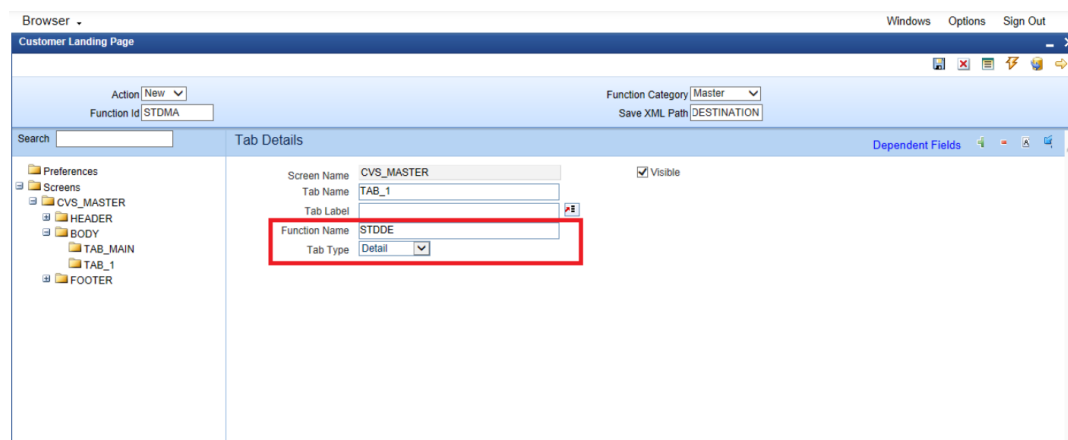
Figure 3-7 Tab Details
