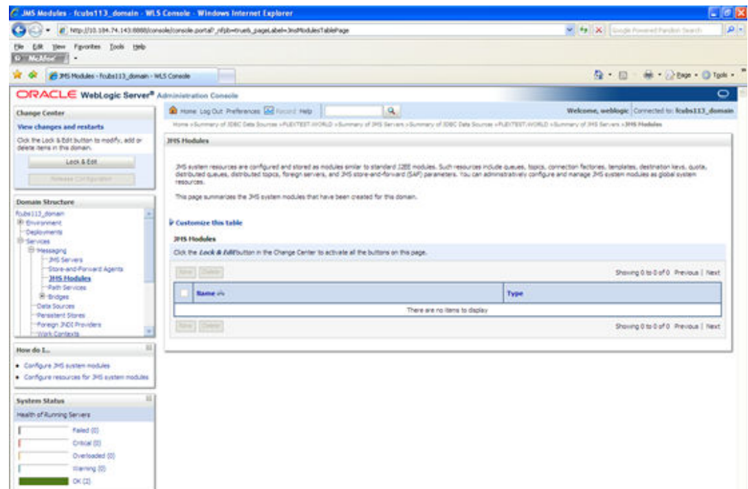
Figure 8-42 Create JMS System Module
