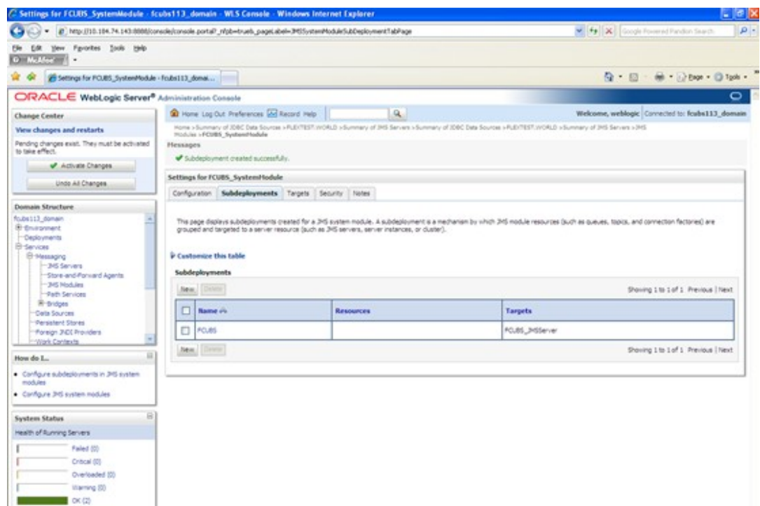
Figure 8-53 FCUBS Subdeployment
