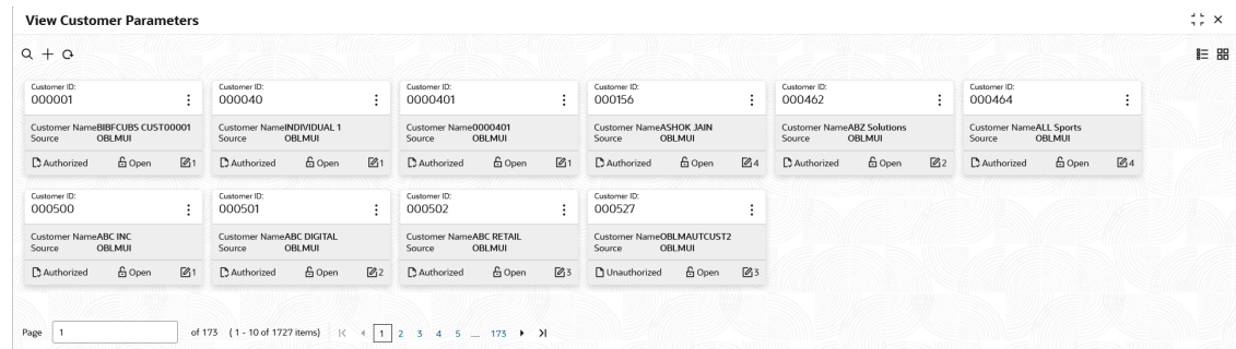
Figure 2-3 Summary Screen
