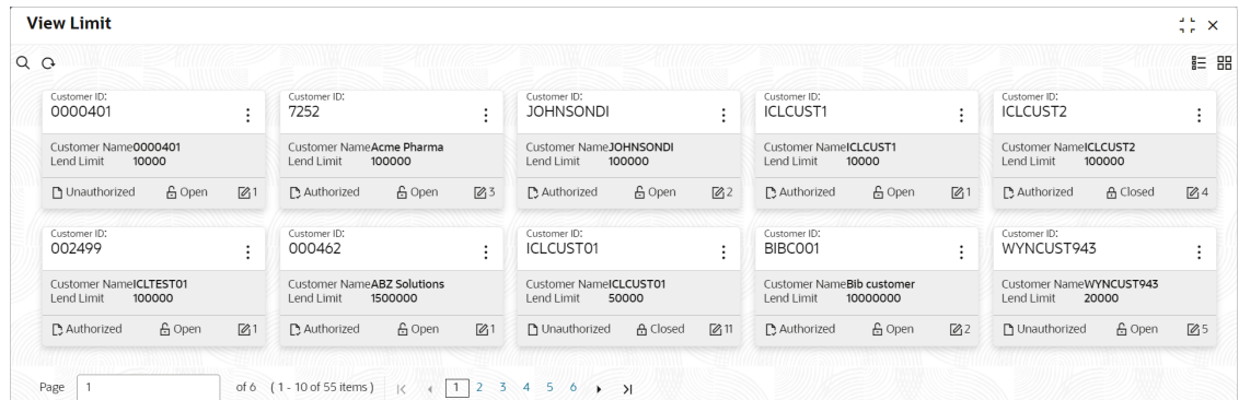
Figure 3-1 Tile View
