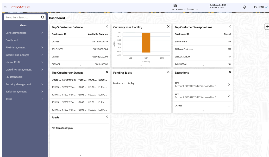
Figure 2-1 Application Environment
