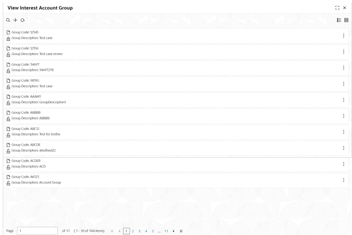
Figure 3-2 List View
