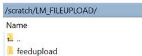
Figure 1-1 File Upload
