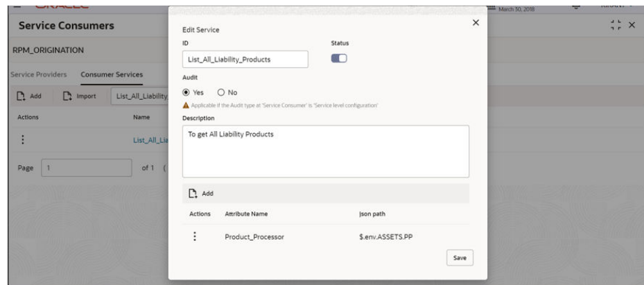
Figure 1-11 Add Attribute
