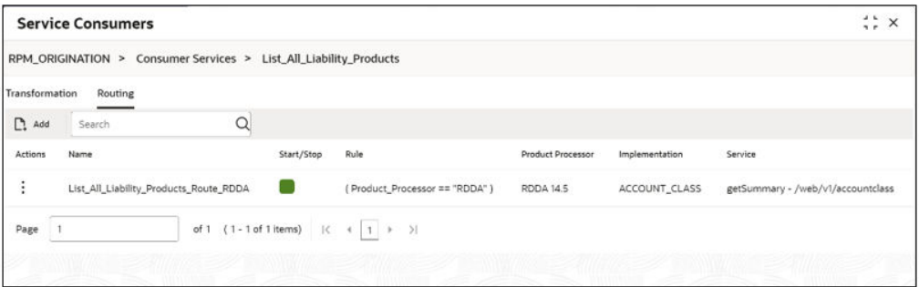
Figure 1-14 Saved route
