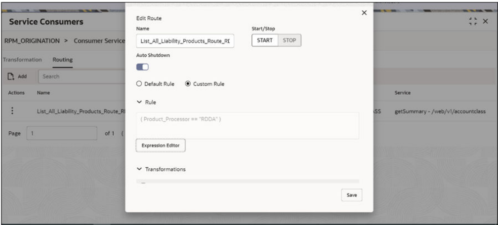
Figure 1-13 Saved Expression
