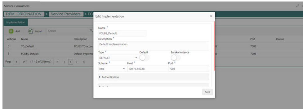
Figure 1-12 Edit Implementation
