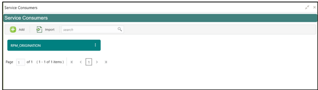
Figure 1-9 RPM Origination
