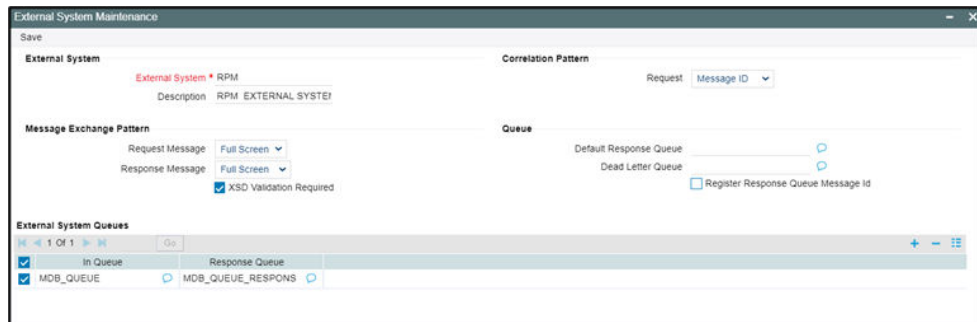
Figure 1-3 External System Maintenance
