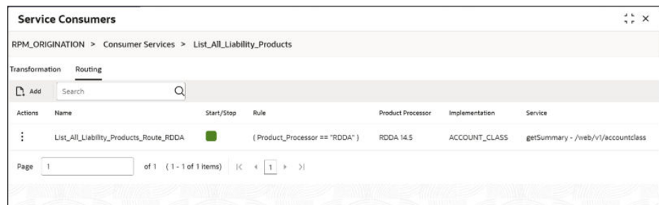
Figure 1-19 Saved route
