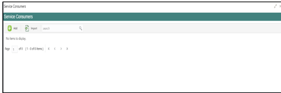
Figure 1-6 Service Consumers
