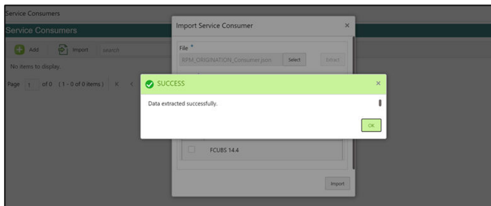
Figure 1-7 Success
