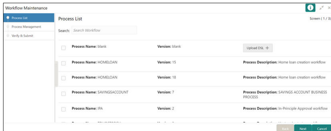
Figure 6-1 Process List
