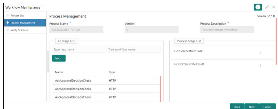
Figure 6-3 Process Management
