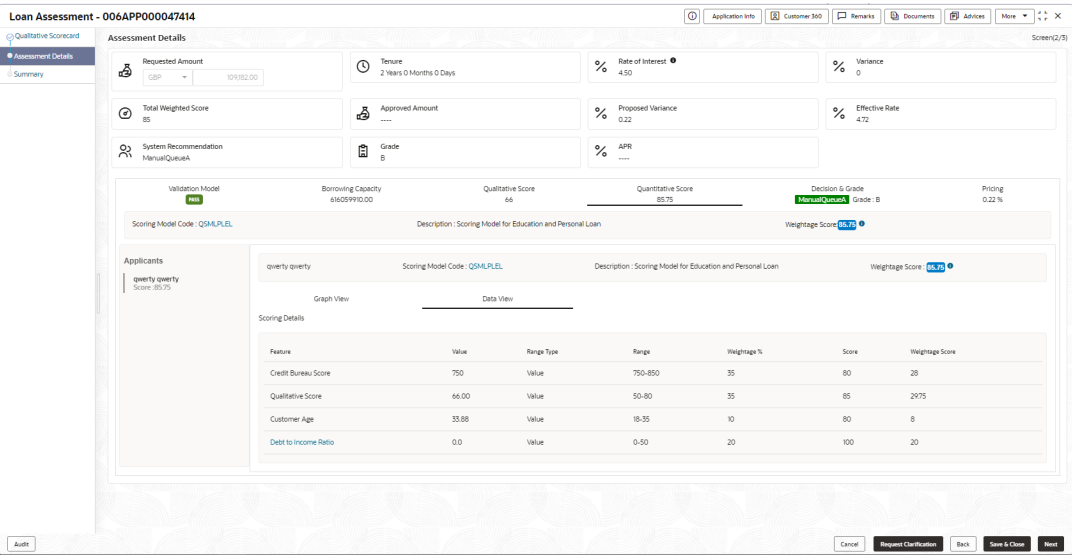
Figure 2-45 Assessment Details – Quantitative Score – Data View
