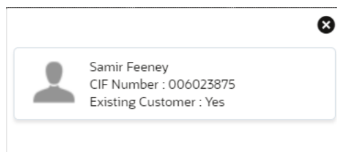
Figure 2-21 Customer 360
