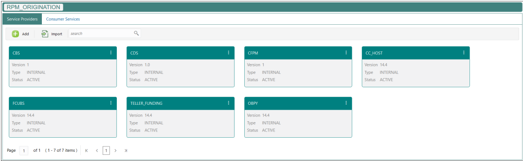
Figure 1-2 RPM_ORIGINATION
