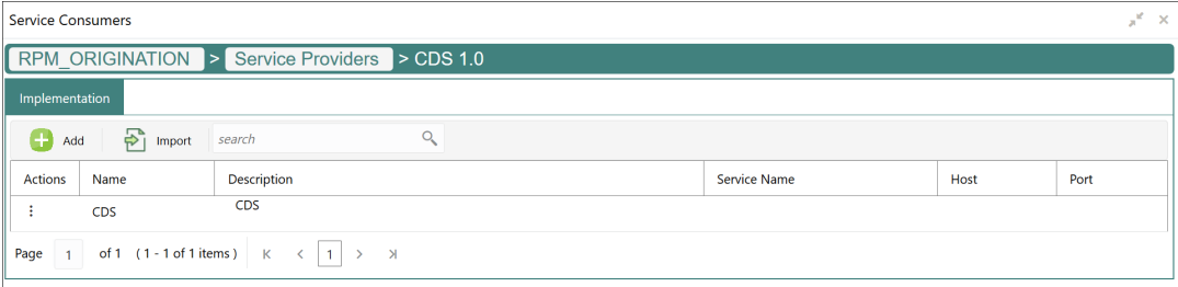
Figure 1-3 RPM_ORIGINATION - CDS
