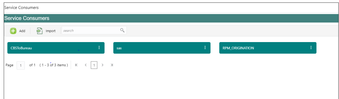
Figure 1-1 Service Consumers
