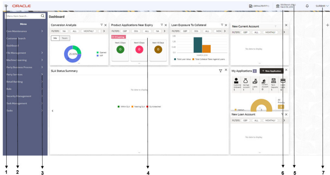
Figure 4-1 Application Environment
