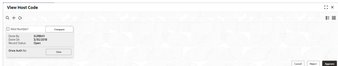
Figure 5-6 Authorization
