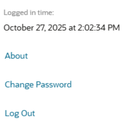
Figure 3-2 Log Out
