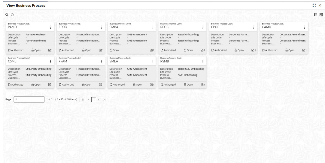
Figure 5-1 Tile View
