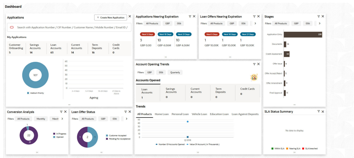
Figure 4-2 Dashboard
