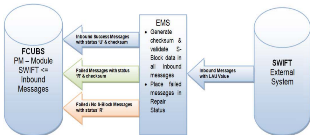
Figure 4-8 Detailed Processing Logic for Incoming SWIFT LAU
