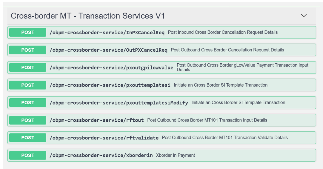
Figure 1-7 Select the Required YAML
