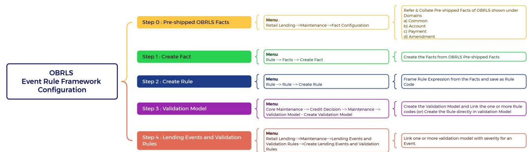
Figure 2-83 Event Rule Framework Configuration
