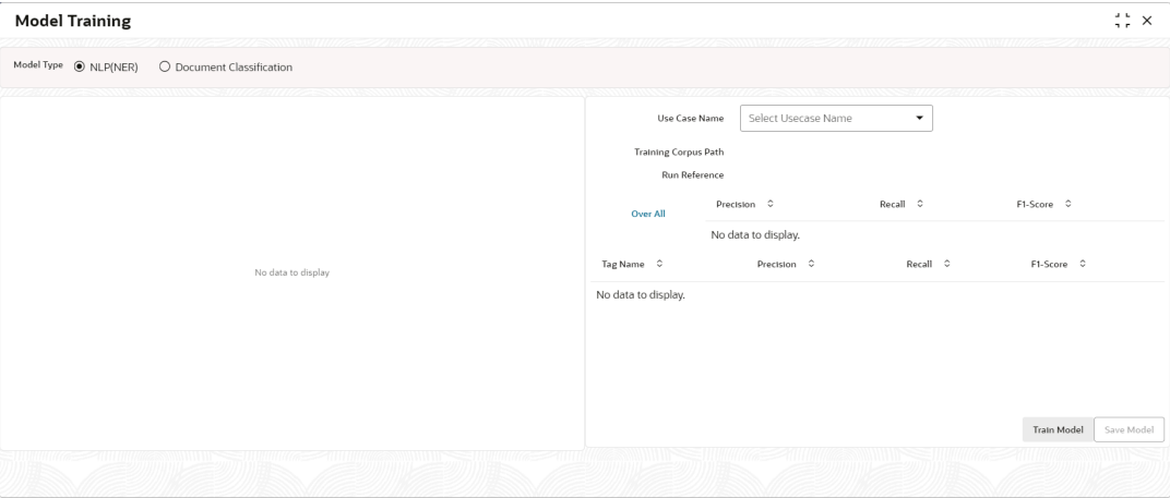
Figure 6-5 Model Training
