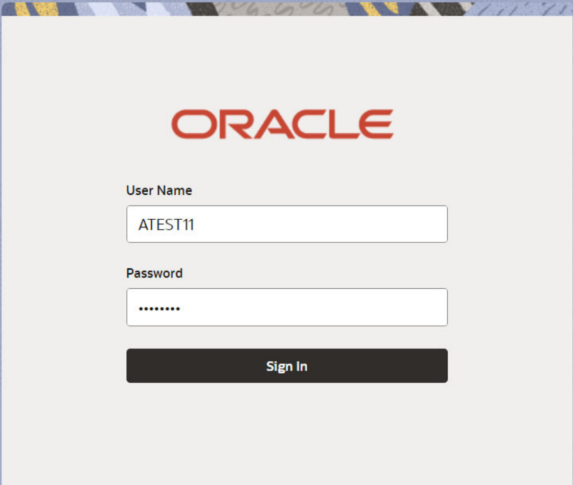
Figure 2-2 LogIn Screen
