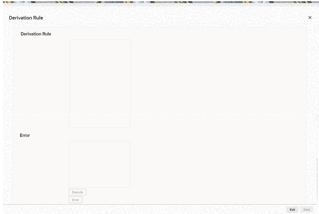
Figure 1-3 Derivation Rule
