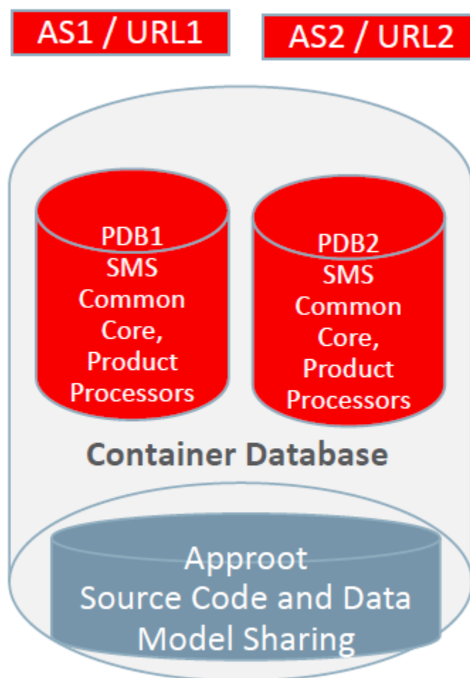
Figure 2-1 Shared Application
