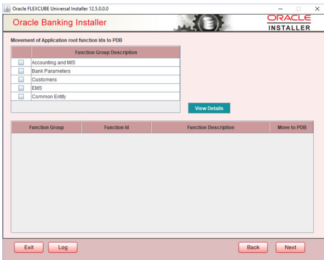
Figure 4-20 View Details
