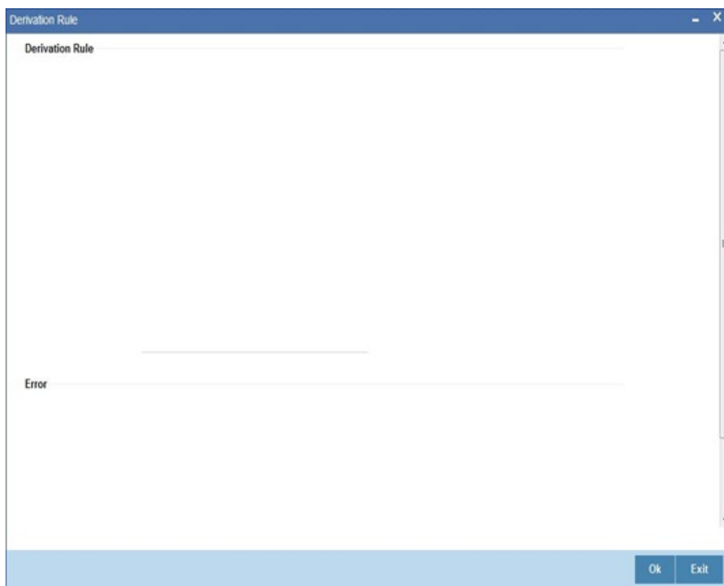
Figure 1-3 Derivation Rule
