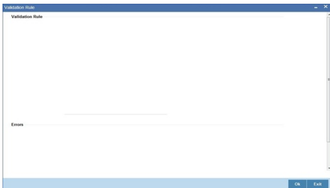
Figure 1-4 Validation Rule
