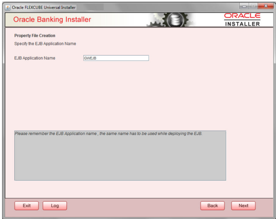
Figure 1-28 Oracle Banking Installer- EJB Application Name
