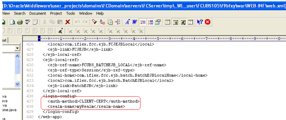
Figure 2-1 web.xml file
