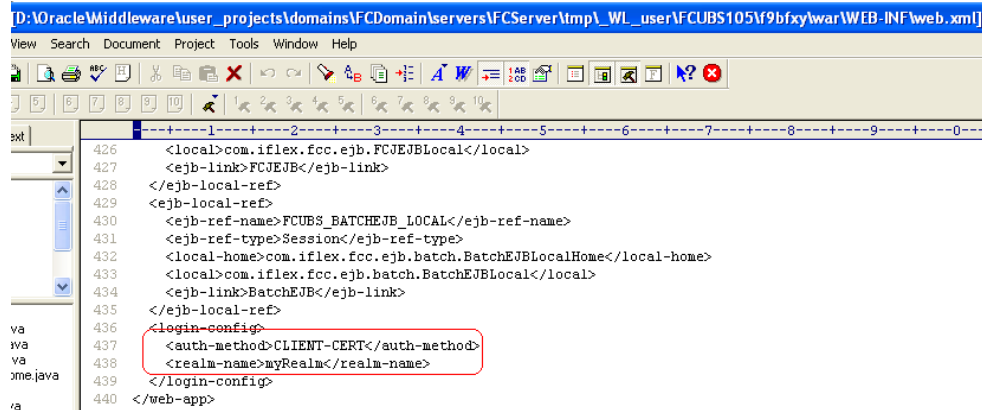
Figure 2-1 web.xml file
