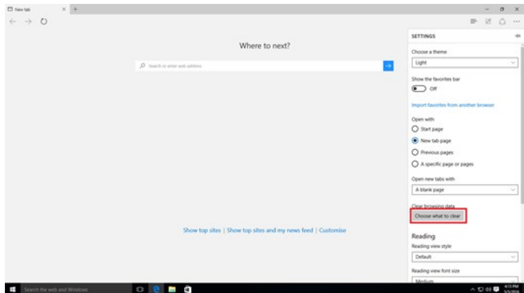
Figure 3-1 Settings pane
